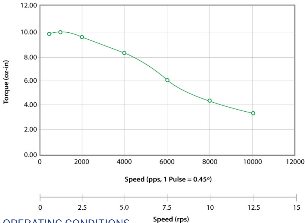
Z417-11-09 (0.9° Step Motor) 24VDC, 0.8 Amp/Phase, Bipolar, 1/2 Stepping
